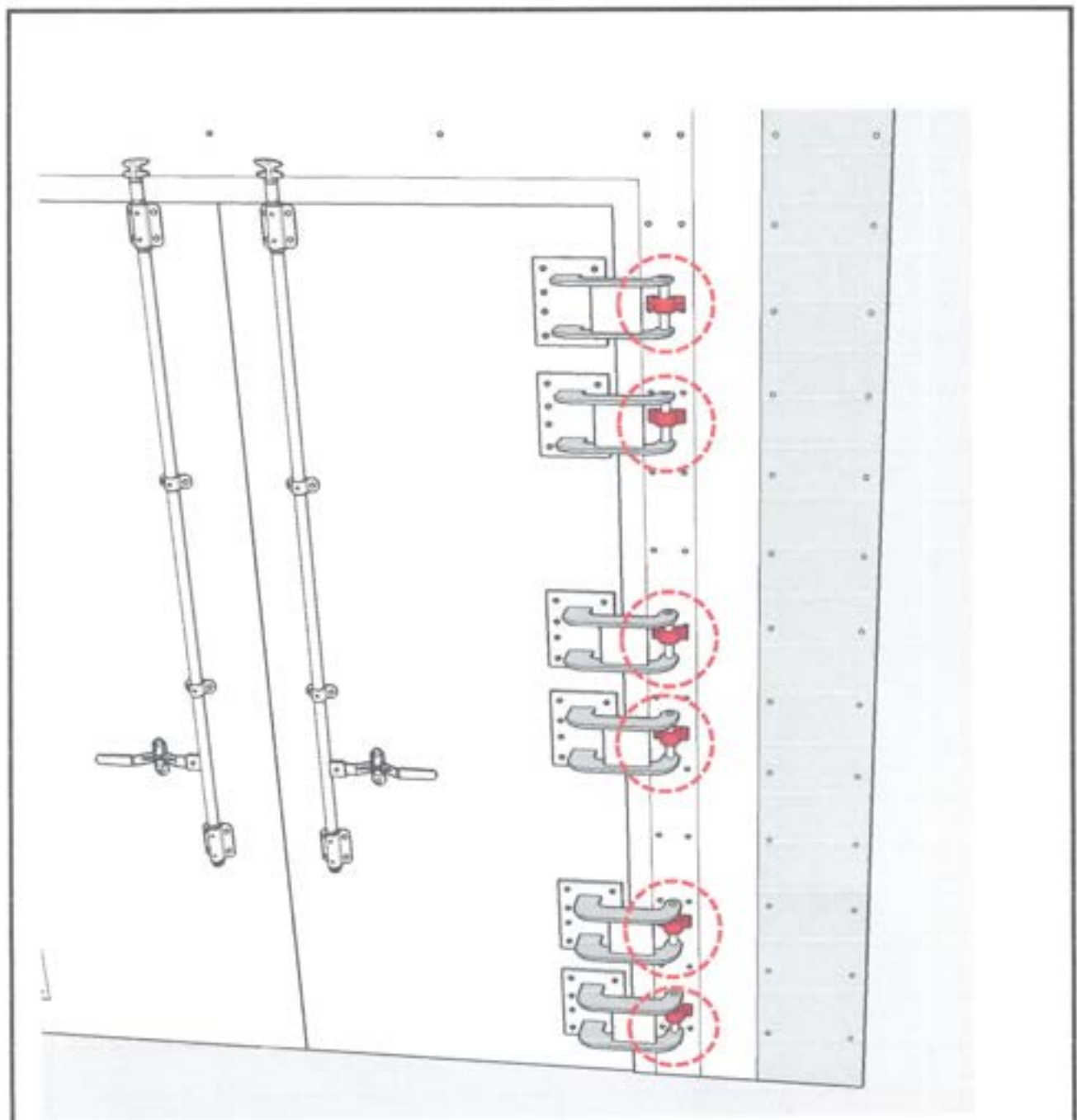
Figure 1. Pillow Bearing Hinges that needs to be repaired
