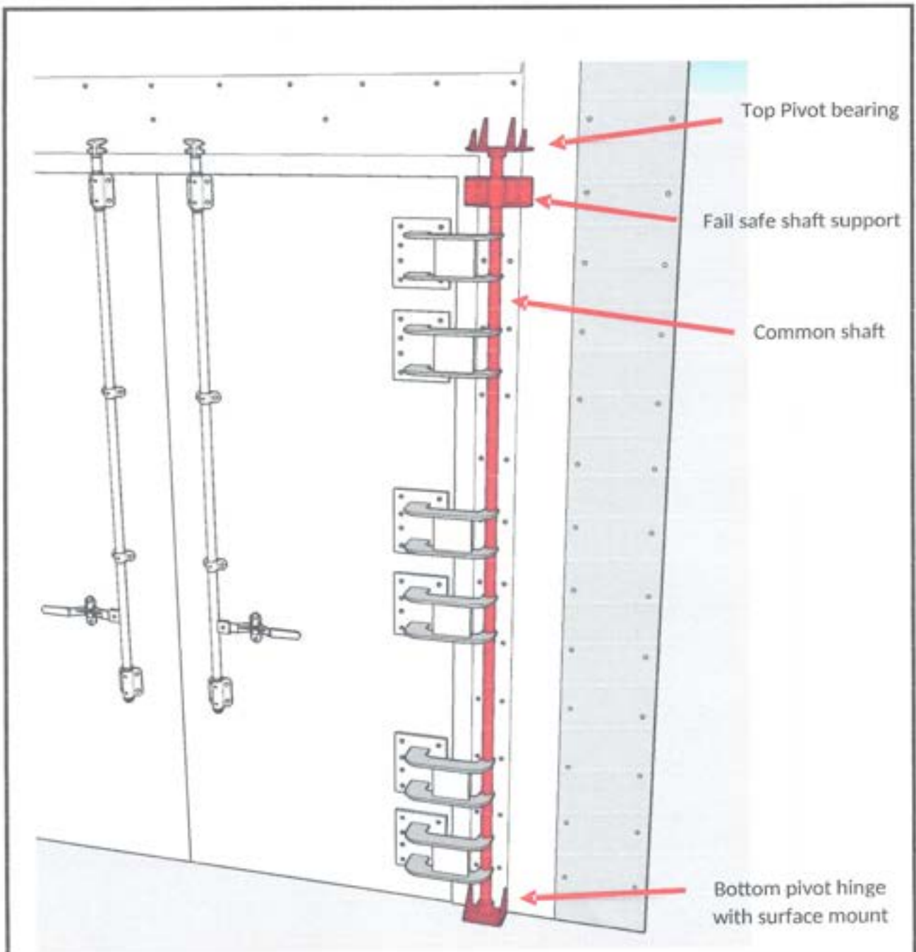
Figure 2. Required repairs for the oven doors
